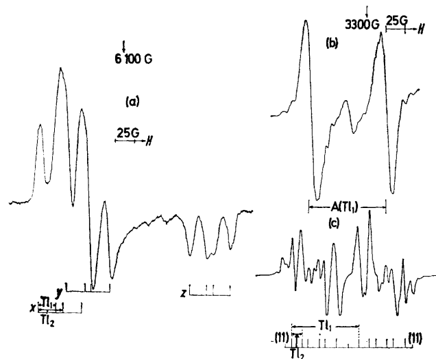
FIGURE 1 First derivative X-band e.s.r. spectra for thallium(III) acetate after exposure to 60 Co \gamma -rays at 77 K, showing (a) high-field features assigned to Tl III , (b) features assigned to \text{D}_2\text{CCO}_2^- at ca. 77 K, and (c) features assigned to \text{H}_2\text{CCO}_2^- at ca. 130 K
