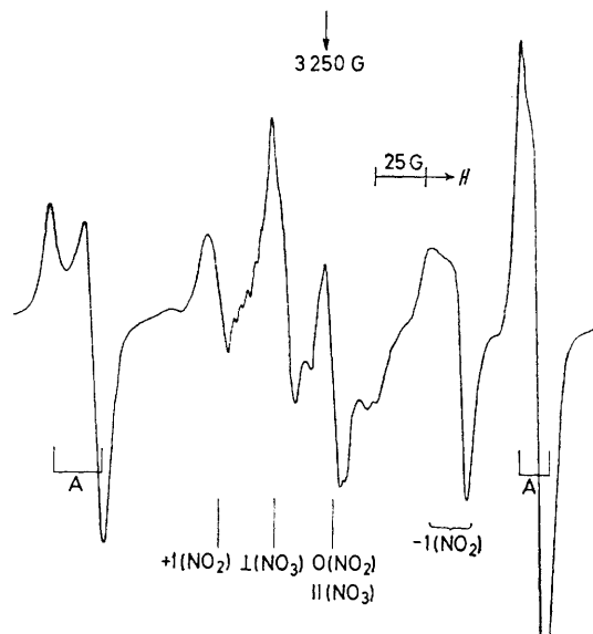
FIGURE 2 First derivative X-band e.s.r. spectra for thallium(III) nitrate after exposure to 60 Co \gamma -rays at 77 K, showing features assigned to \text{NO}_2 and \text{NO}_3 radicals together with species A discussed in the text
